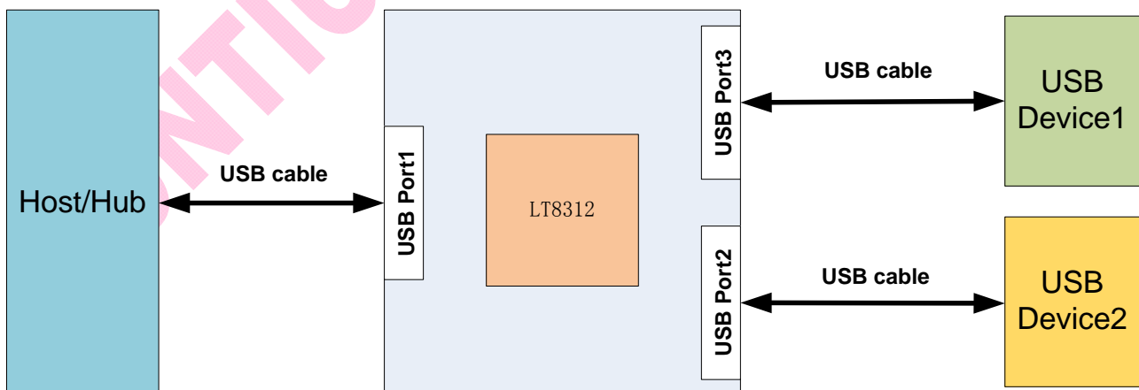
Figure 1. Application Diagram
